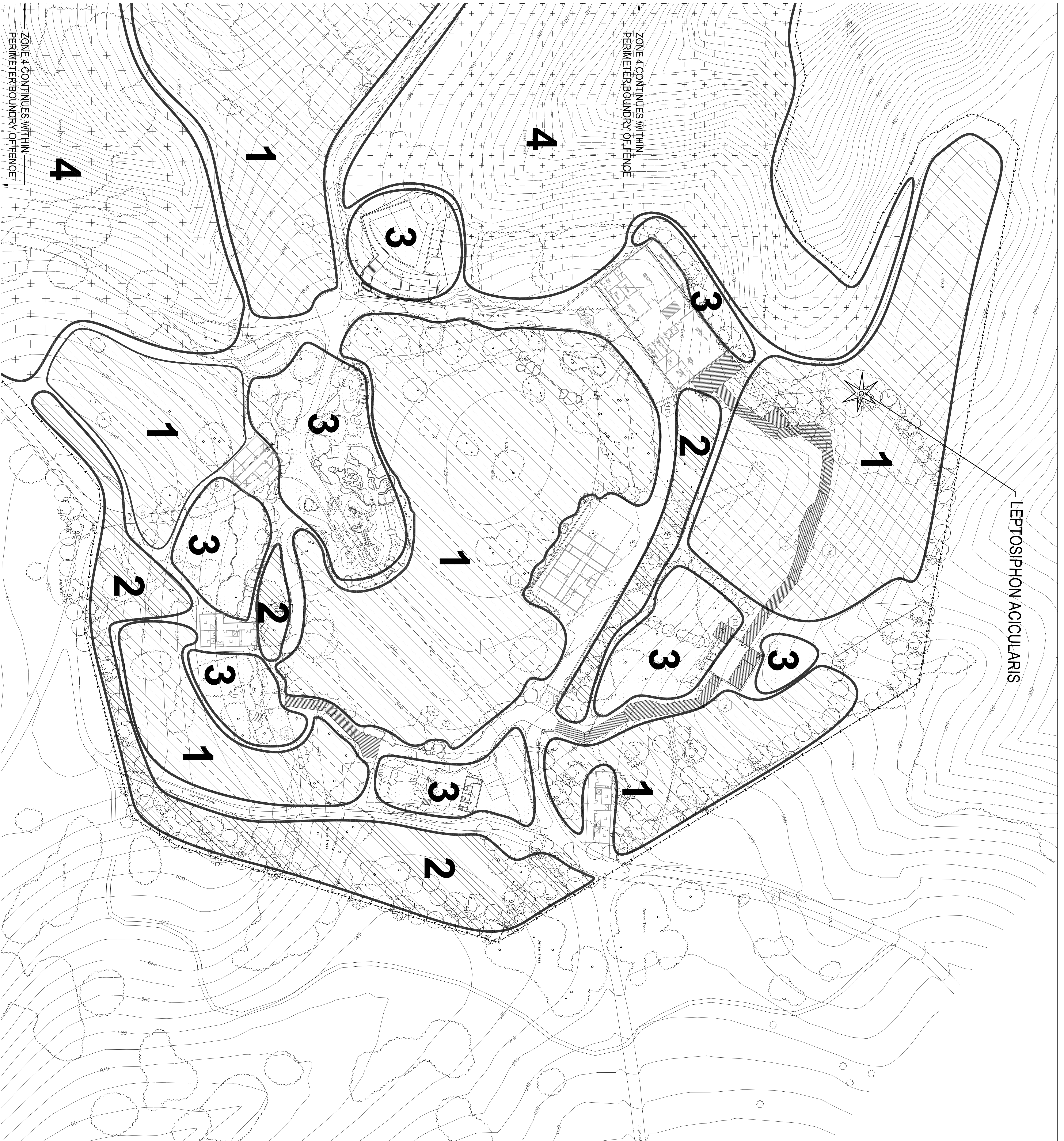
SCHEMATIC PLANTING PLAN DIAGRAM SCALE: 1" = 50'-0"
